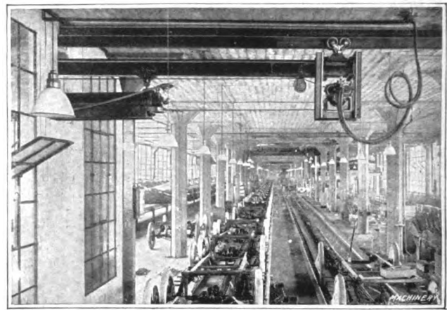
Fig. 11—In the trolley rail extension (Fig. 10), the air cylinder actuates the hoist and the pneumatic motor runs the extension out so that the hoist can pick up its load and carry it back into the shop, where the auto body is put on a conveyor and carried to the assembling department
